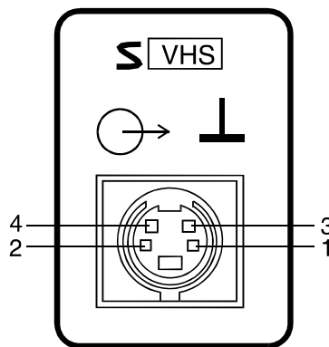
Figure 8.- S-VHS socket
